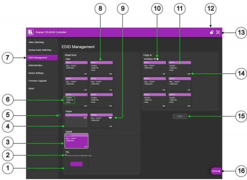
Figure 12: EDID Page
