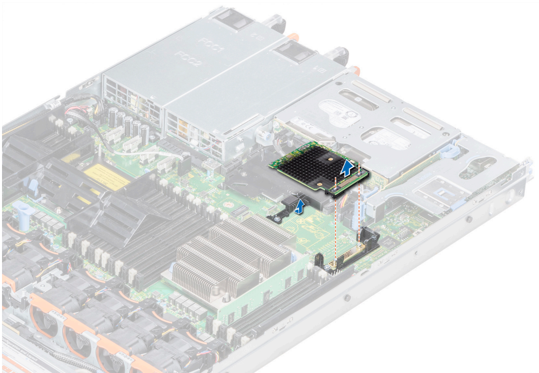
Figure 22. Remove HBA350i MM
