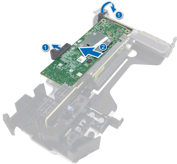
Figure 19. Remove the HBA350i Adapter
