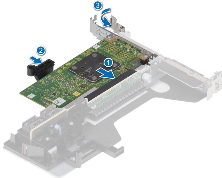
Figure 12. Install the HBA355e Adapter
