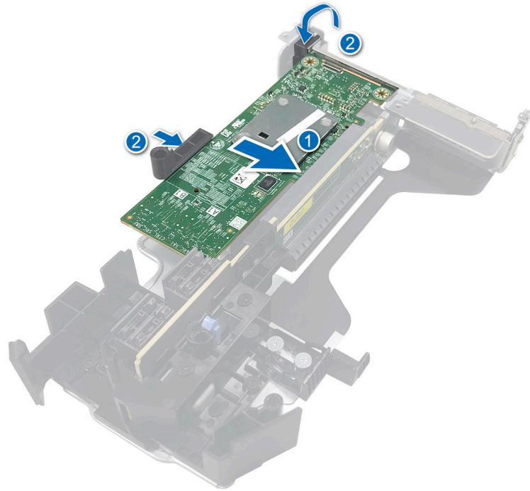
Figure 20. Install the Dell HBA350i Adapter
