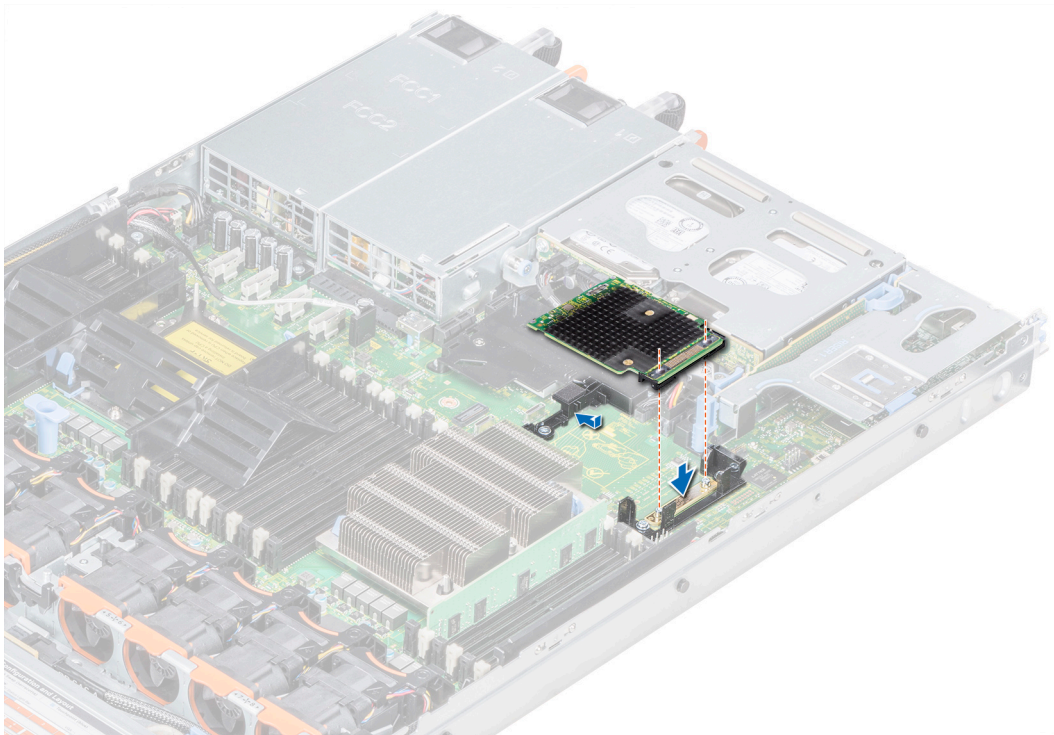
Figure 23. Install Dell HBA350i MM
