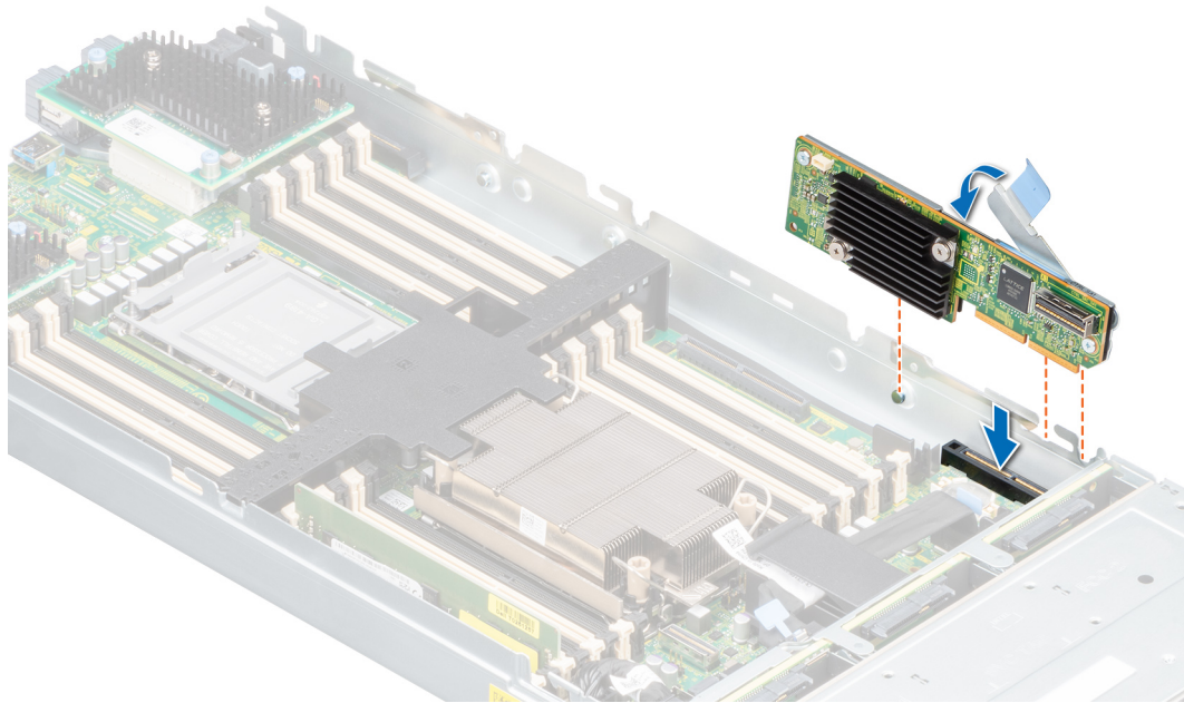
Figure 18. Install Dell HBA350i MX
