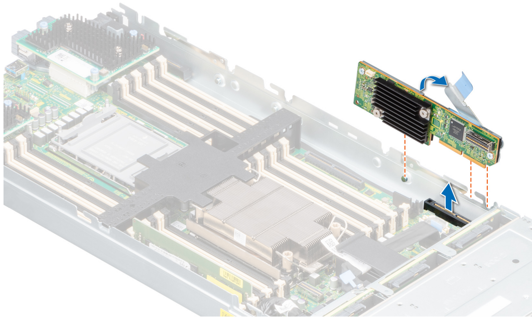
Figure 17. Remove Dell HBA350i MX
