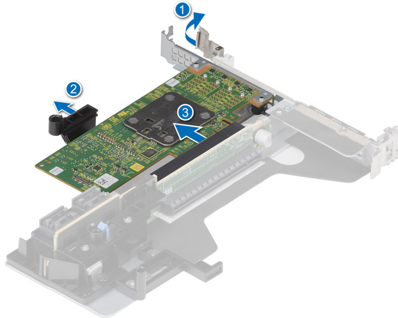
Figure 11. Remove the HBA355e Adapter
