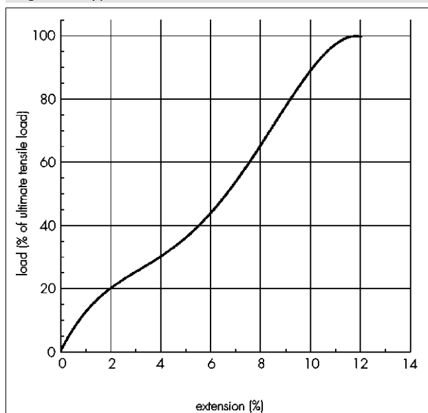
Figure 6 Typical load extension curve
