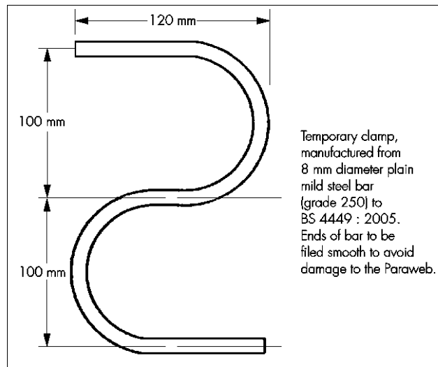
Figure 2 Steel 'S' clamp
