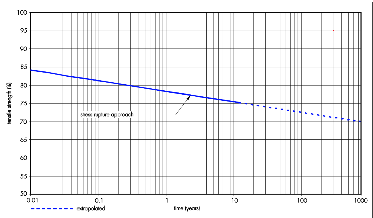
Figure 7 Regression line for life expectancy at constant stress defined by percentage of characteristic short-term tensile strength at 20°C
