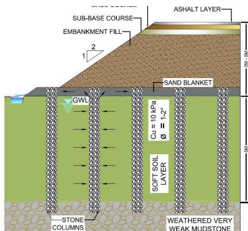
Original solution of ground improvement with stone columns
