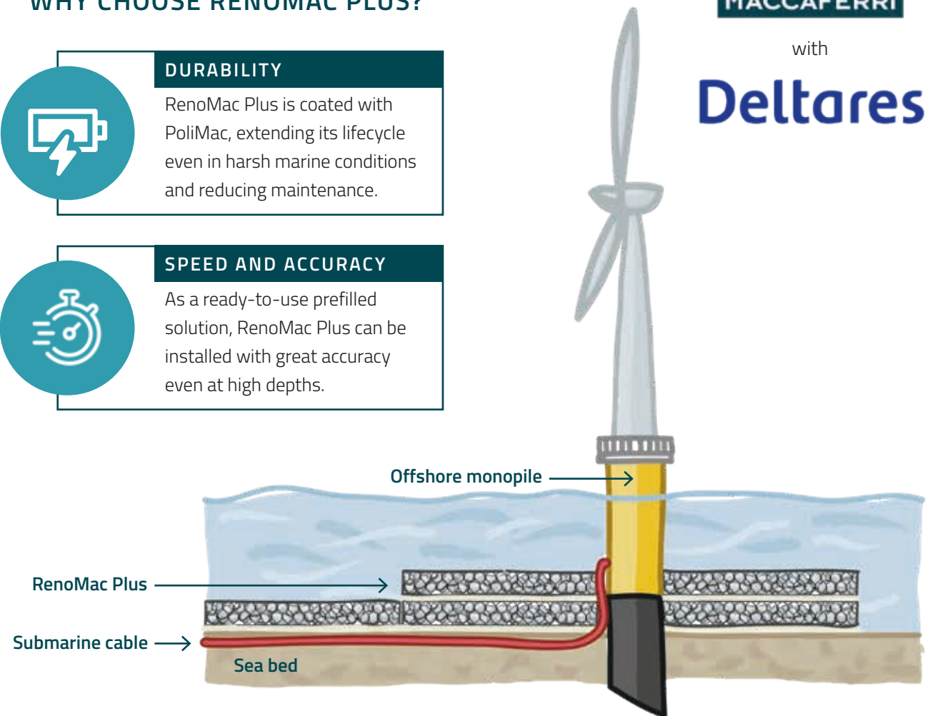
RenoMac Plus layout for protection of offshore monopile foundation and submarine cables
