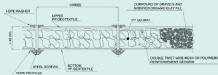
Remedial Filtering Mattress (RFM)
