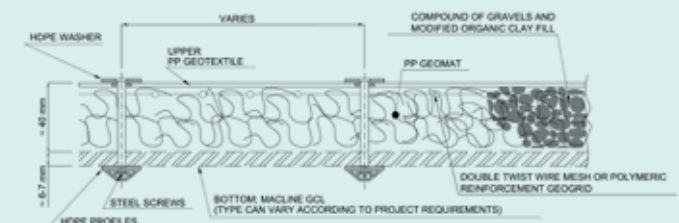
Remedial Sealing Mattress (RSM)
