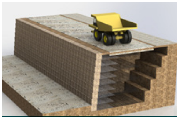
Terramesh® reinforced soil
