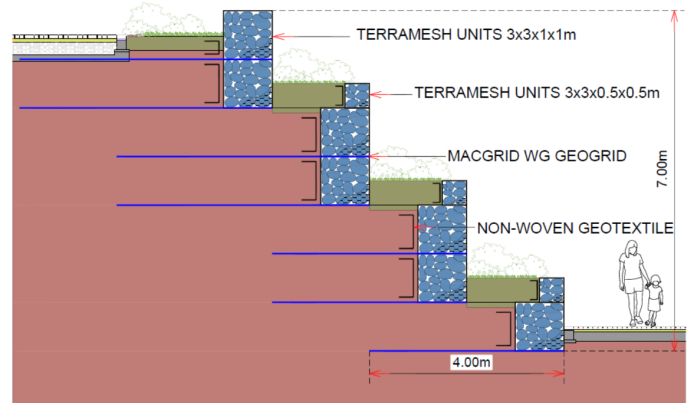
Sectional details of tiered Terramesh MSE wall
