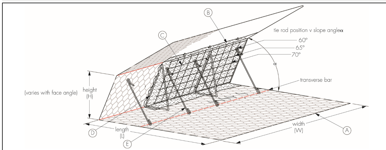
Figure 1 The Maccaferri Green Terramesh System — Typical composition of units
