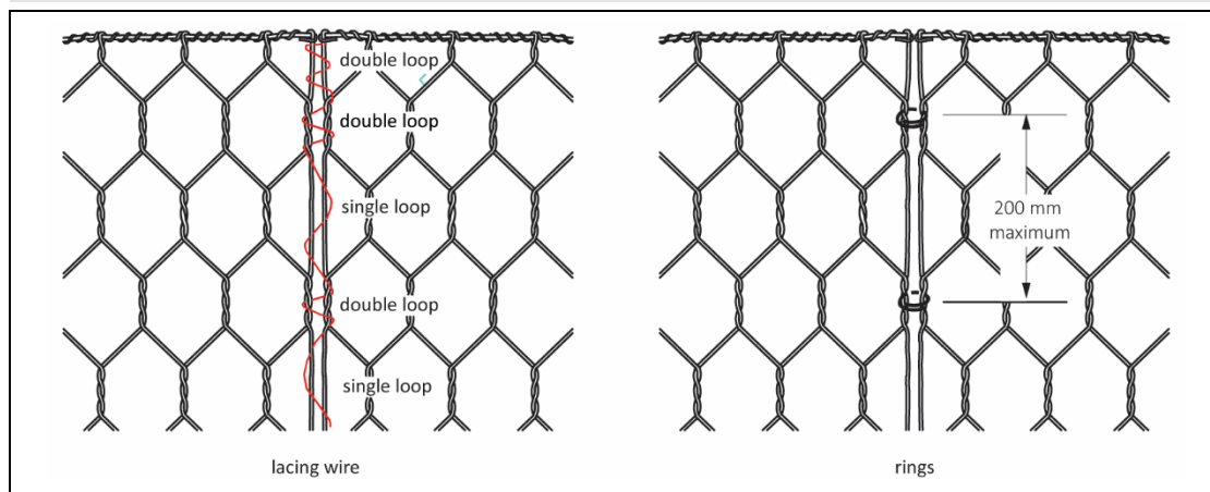
Figure 4 Typical Face panel connection detail
