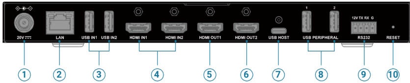
Figure 2: Rear Panel
