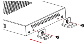
Figure 3: Installing Brackets
