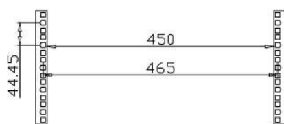
Installation dimension
