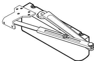
Parallel Arm Installation
