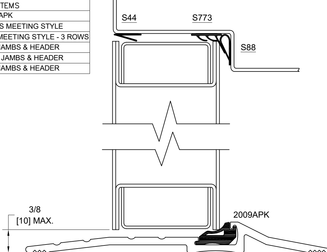
HEADER/JAMB VIEW VIEW OF FRAME AND DOOR PERIMETER
