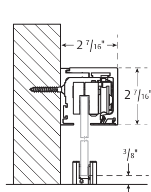
WALL MOUNT
