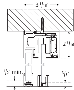
CEILING MOUNT
