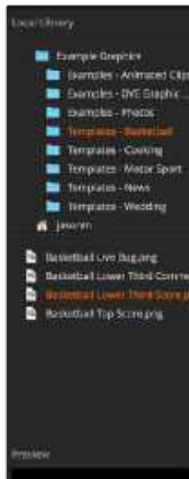
Browse window
