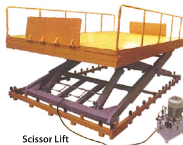
Scissor Lift
